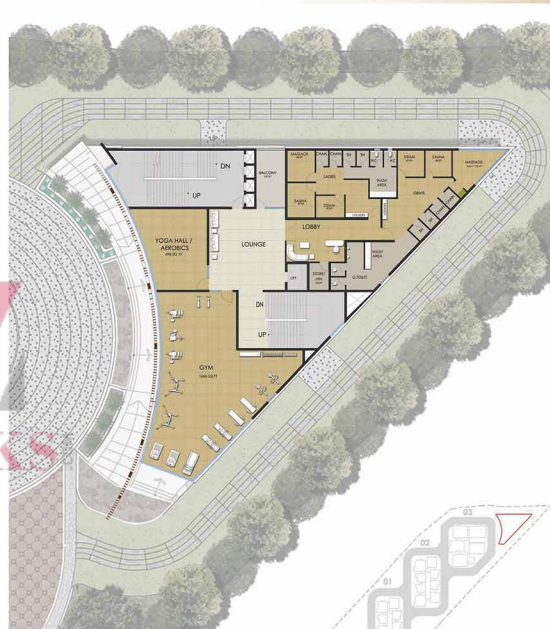
CLUB HOUSE FIRST FLOOR PLAN
