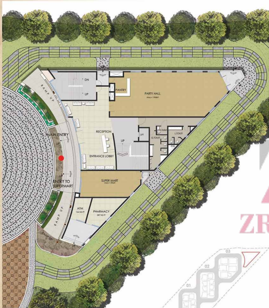
CLUB HOUSE GROUND FLOOR PLAN
